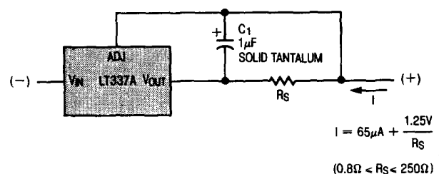
Current Regulator
